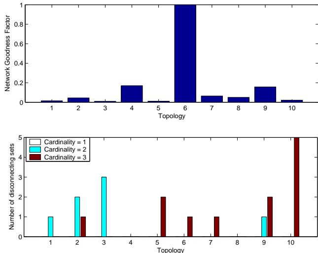
Fig. 9. Top graph shows the network goodness factors while the bottom graph shows the disconnecting sets for different topologies
