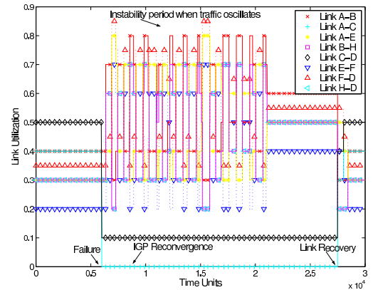
Figure 6: Link loads for various links in the IP network with alternate probe spacing
