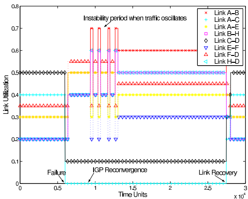
Figure 5: Link loads on various links in the IP network for Scenario 2
